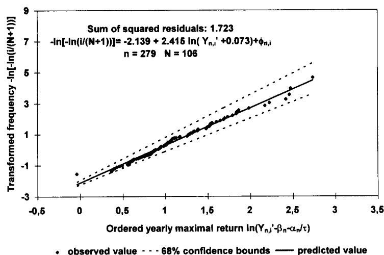
FIG. 3.—Adjustment of the Fréchet distribution to yearly extreme returns. a , minimal returns. b , maximal returns.
